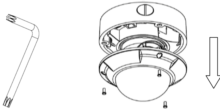
Fig. 2.2.8 Unload the Cover
